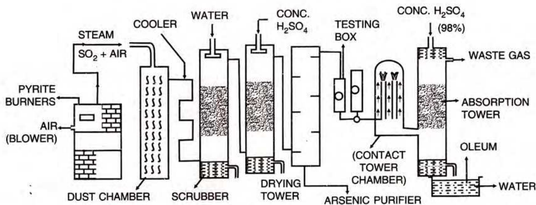
Fig. 11.1. Contact process for the manufacture of H_2SO_4 acid
