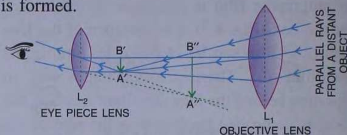
Fig. 4.7 Ray diagram of a telescope
